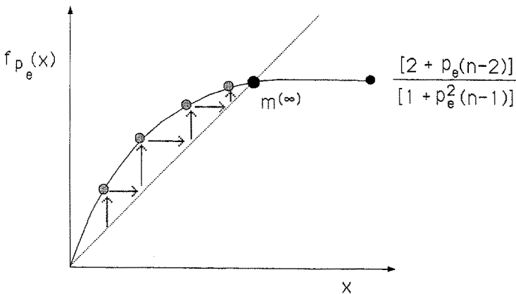
Fig. 7. Magnetization dynamics: the supercritical case
