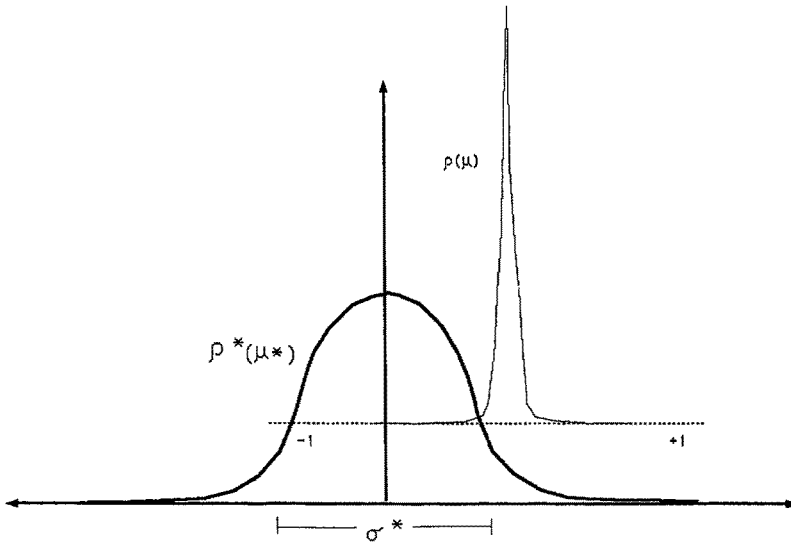
Fig. 4. The solution near p_G . Gaussian nature of the solution illustrated above. q(\mu) is the “actual” solution. The rescaled solution, q^*(\mu^*) \equiv \sqrt{\Delta} q(\mu/\sqrt{\Delta}) , is Gaussian to lowest order. The rescaled width, \sigma^* , is a (computable) number of order unity
