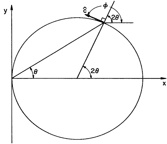
FIG. 10. Why \phi=2\theta+\pi/2 is a natural pattern for filling a circle with tangential boundary conditions.
