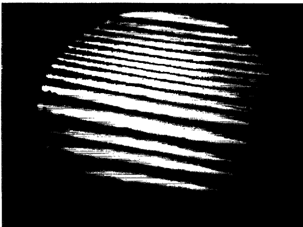
FIG. 3. Polarized reflection micrograph of the stripe texture. Photo courtesy of N. A. Clark, D. H. Van Winkle, and C. Muzny.
