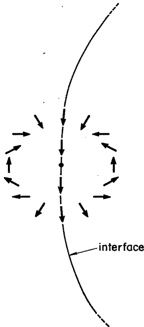
FIG. 9. An s=2 defect. \phi rotates by 4\pi along any simple closed loop encircling the defect. If the defect lies on a smooth interface, then only half the loop exists. \phi rotates by 2\pi along this half path, making \phi continuous along the interface.
