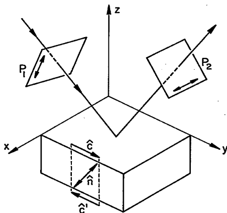
FIG. 1. Schematic of the experiment. The smectic film lies in the x-y plane. The film is viewed by reflection between crossed polarizers P_1 and P_2 . The molecular optical axis is \hat{n} —the molecule shown lies in the y-z plane. The order parameter \hat{c} points towards the tops of the tilted molecules, and lies in the x-y plane. Consequently, when the film is viewed from below, the order parameter \hat{c}' is the reverse of \hat{c} .
