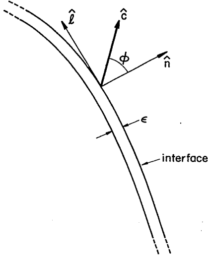
FIG. 12. Definition of the coordinate system for surface terms. Derivatives of \phi with respect to \hat{n} diverges as \epsilon \rightarrow 0 .
