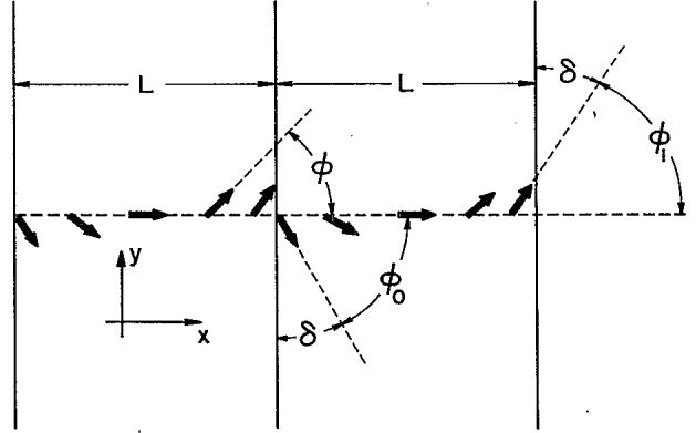
FIG. 6. Geometry of the stripe pattern, showing two stripes separated by a defect line. The order parameter \hat{c} makes an angle \phi(x) with the x axis. At the left-hand edge of a stripe \phi = -\pi/2 + \delta , and at the right-hand edge \phi = \pi/2 - \delta .
