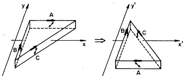
FIG. 5. Transformation of the order parameter under a 180^\circ rotation about \hat{\mathbf{x}} . The x components of the in-plane projections of the molecular axes are reversed on rotation, but the y components are not.
