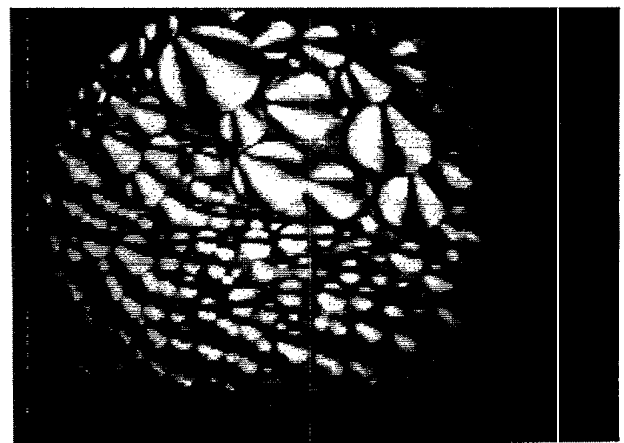
FIG. 2. Polarized reflection micrograph of the droplet texture. The polarization axes are parallel to the edges of the picture. The diameter of the illuminated region is roughly 0.24 cm. Photo courtesy of N. A. Clark, D. H. Van Winkle, and C. Muzny.
