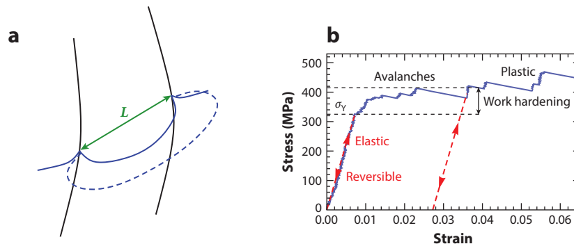
Figure 3 (a) Pinned dislocation line. (b) Avalanches and work hardening in a micropillar stress-strain curve.
