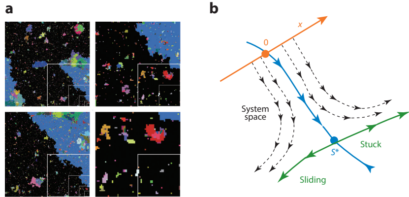
Figure 10 (a) Self-similarity and (b) renormalization group flow diagram.
