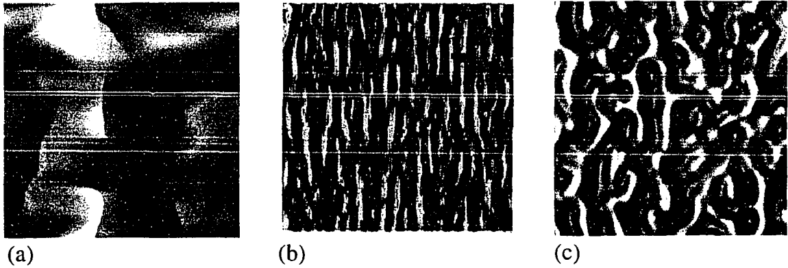
Figure 7.4: (a) Cusps formed with one slip system. Plastic distortion tensor \beta_{yx}^P formed by climb-free evolution of a Gaussian random initial state of edge dislocations pointing along \hat{z} with Burgers vector along \pm\hat{x} . Notice that walls do not form with one slip system, only cusps in the distortion tensor; compare to [4]. (b) Continuum of walls. The dislocation density tensor \rho_{zx} evolved allowing both glide and climb from a random initial state of edge dislocations along \mathbf{t} \parallel \hat{z} with \mathbf{b} \parallel \hat{x} . Notice that the dislocations arrange themselves into small-angle tilt boundaries at the lattice scale, but do not coarsen; compare to [5]. (c) Cell walls in a climb-free simulation with two active slip systems \rho_{zx} and \rho_{zy} , edge dislocations perpendicular to the simulation. Notice the walls separating cells. Here the smaller length scale reflects the smaller Gaussian correlation length we used for the initial conditions. Also, we only show \rho_{zx} , so the cell walls appear incomplete; the \rho_{zy} components fill in the gaps leading to a clear cellular pattern.
