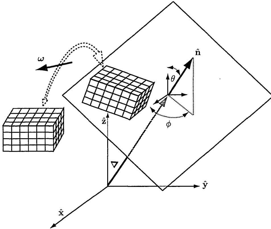
Figure 4.3: A general grain boundary whose normal is \hat{n} positioned at the distance \Delta away from the origin separates two unstrained regions with a relative orientation defined by \omega .
