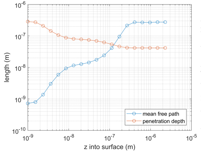
Figure 7: Example field-dependent material parameter input to thermal model framework.
